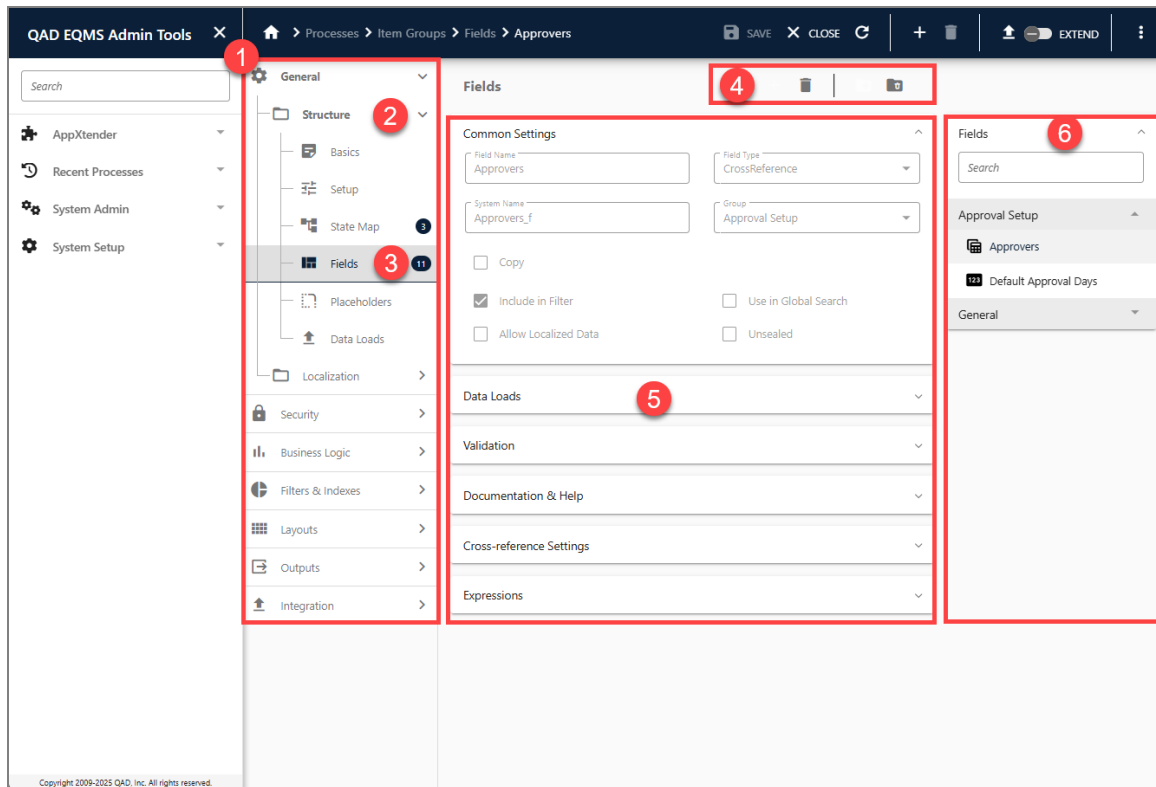
Fig. 3: Process desktop
