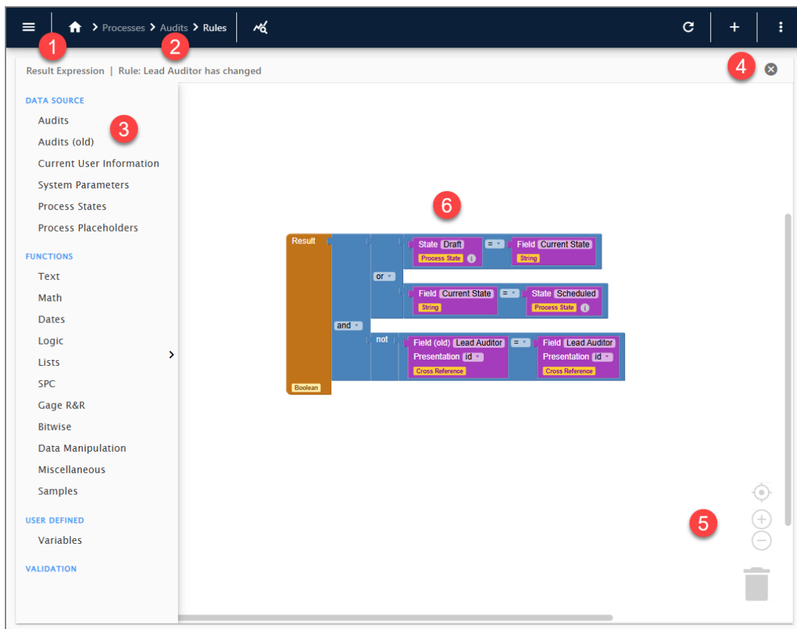
Fig. 31: Expression Builder
