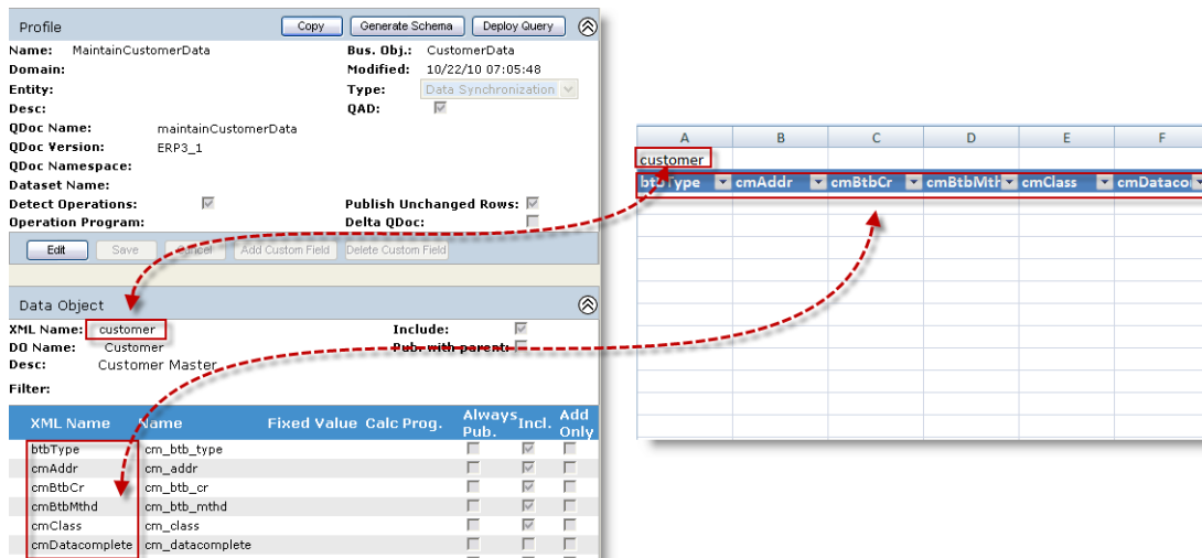
Fig. 3.3 Mapping of Data Object and Field Names
