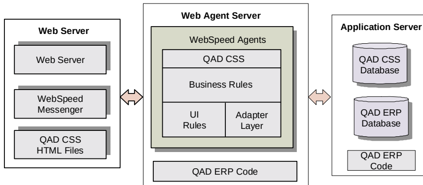
Fig. 1.4 Distributed Deployment of QAD CSS with Separate Database
