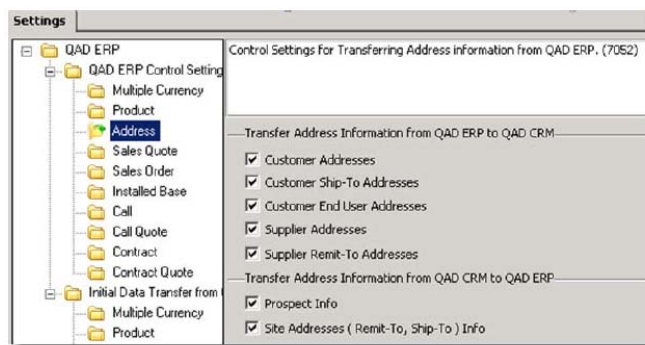
Fig. 11.7 Address (QAD Enterprise Applications – Standard Edition)
