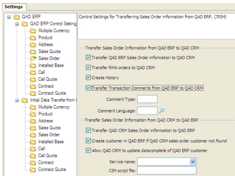
Fig. 11.10 Sales Order
