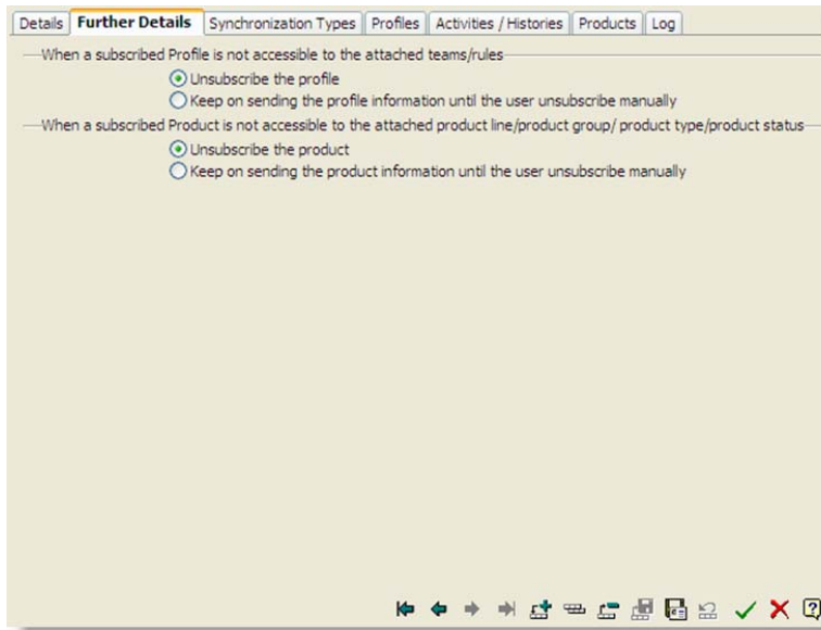
Fig. 12.4 Further Details
