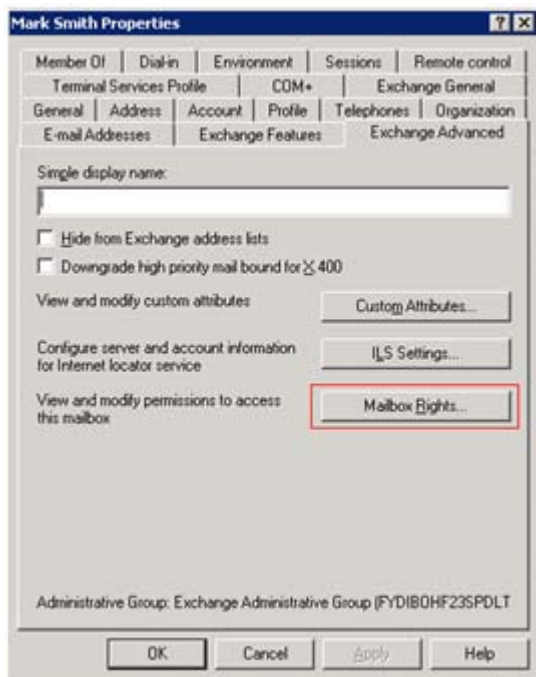
Fig. 14.8 User Properties
