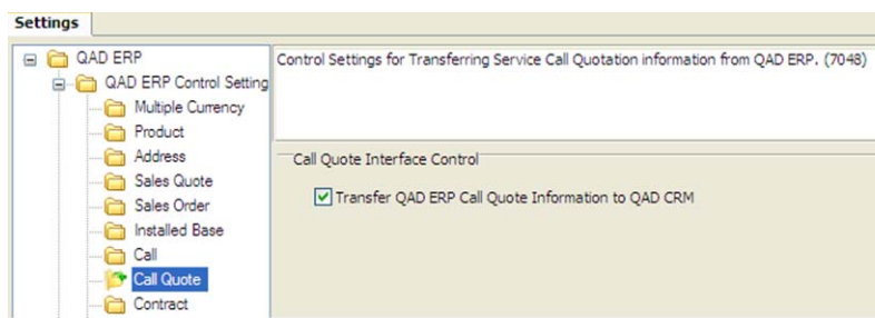
Fig. 11.13 Call Quote
