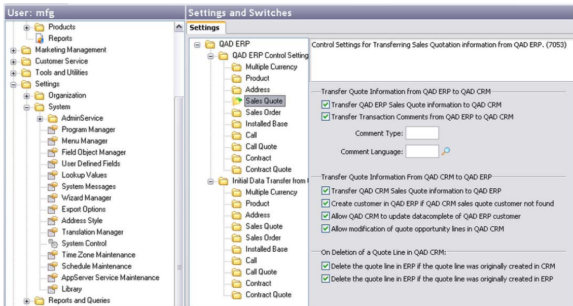
Fig. 11.9 Sales Quote
