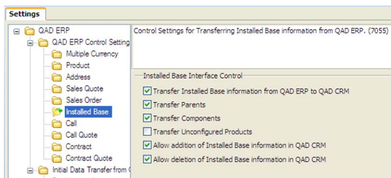
Fig. 11.11 Installed Base
