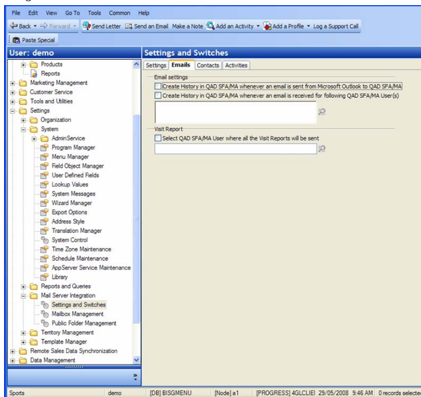
Fig. 14.12 Settings and Switches - Emails
