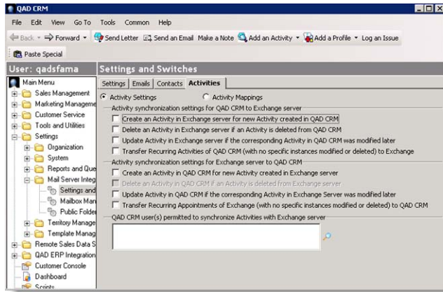
Fig. 14.13 Settings and Switches - Activities Tab
