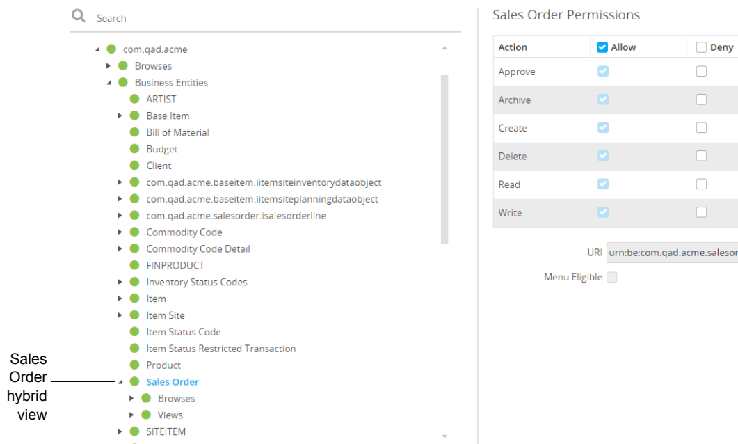
Fig. 7.22 Hybrid View
