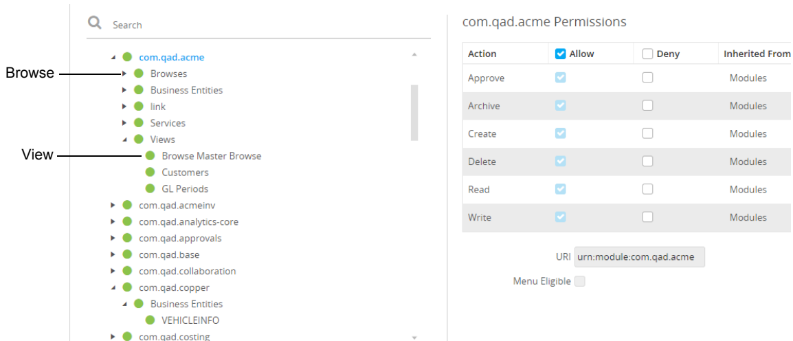
Fig. 7.24 Browse Screen
