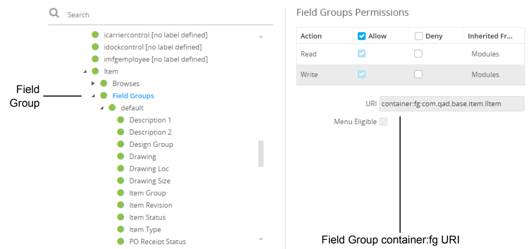
Fig. 7.26 Field Groups
