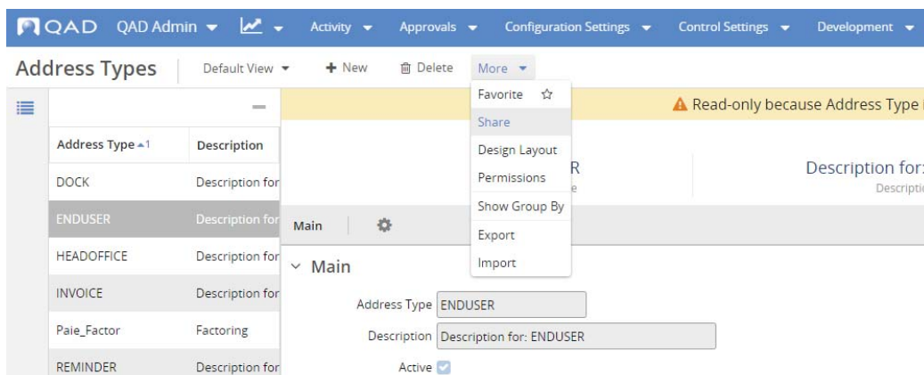
Fig. 7.37 Share Access
