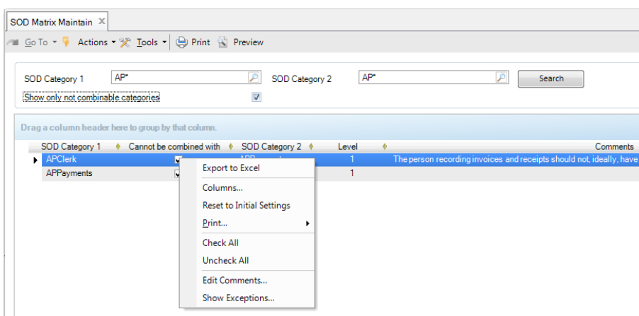
Fig. 9.20 SOD Matrix Maintain, Context Menu
