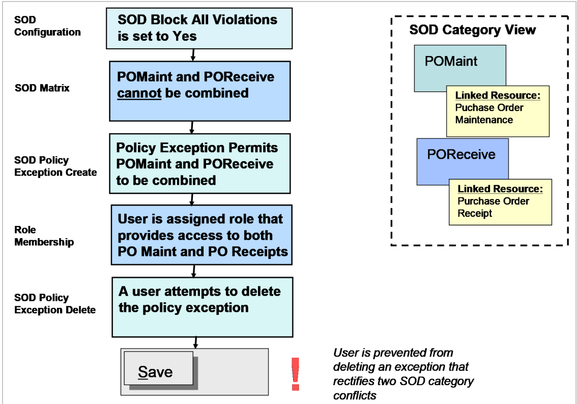
Fig. 8.6 Indirect Segregation of Duties Violation
