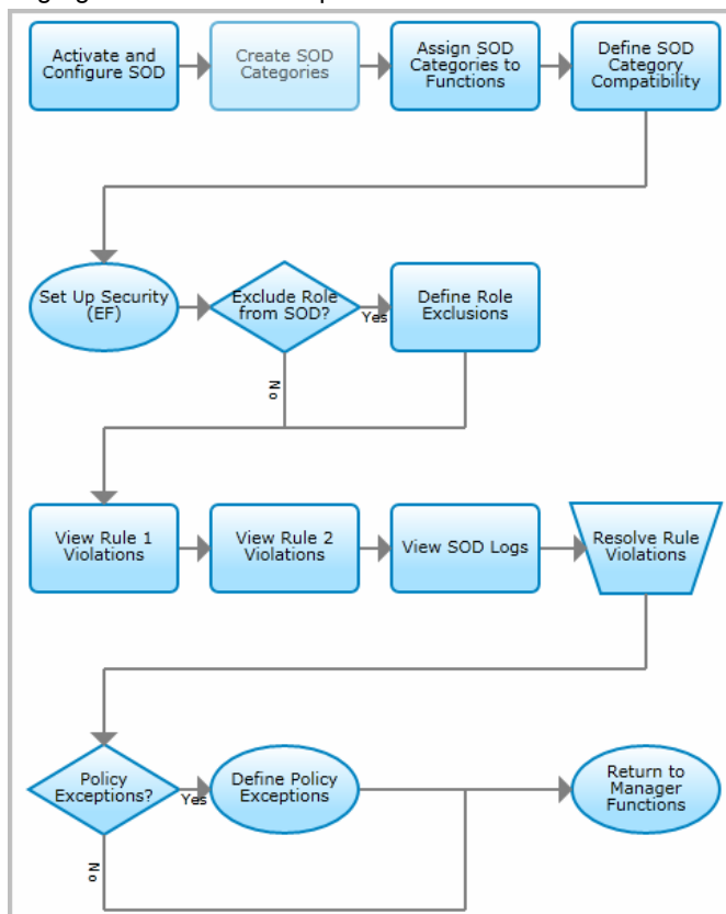
Fig. 8.3 Segregation of Duties Setup Flow
