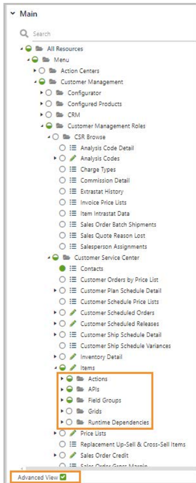
Fig. 6.12 Role Permissions Tree
