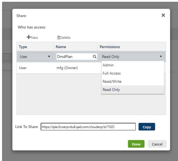
Fig. 6.33 Define Share Access
