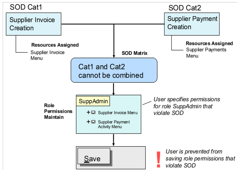
Fig. 8.4 Role Permissions Validation
