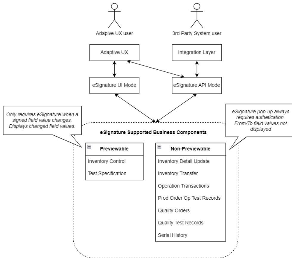
Fig. 9.12 User Interaction with E-Signature Modes and Business Components
